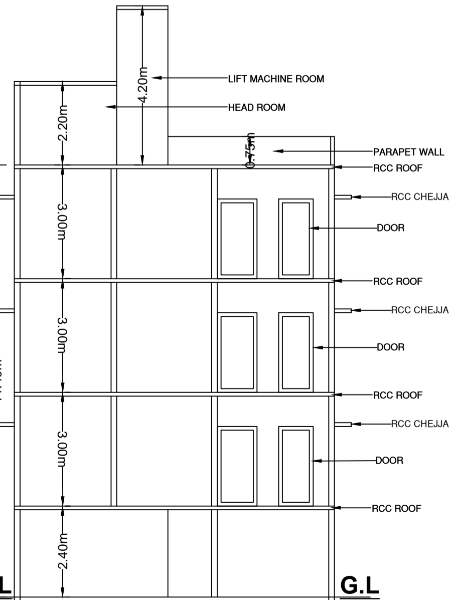
SECTION @ AA
